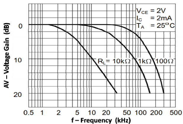
Fig 13 Frequency Response
