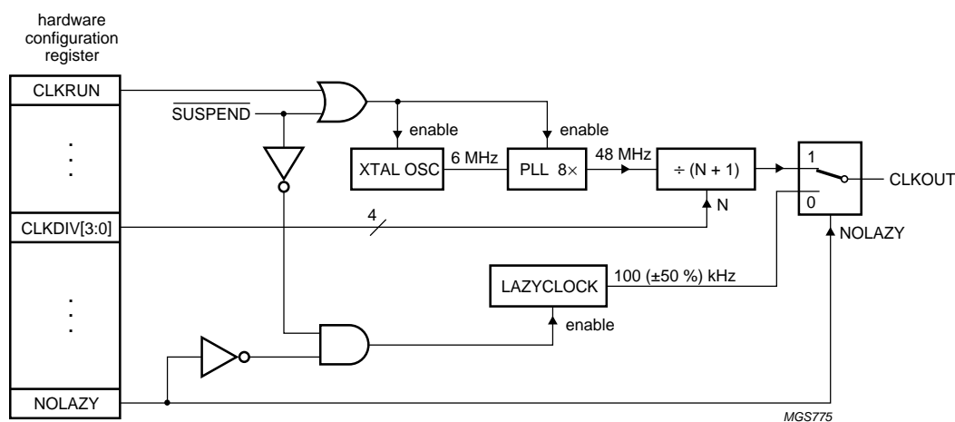
Fig 47. Oscillator and LazyClock logic.
