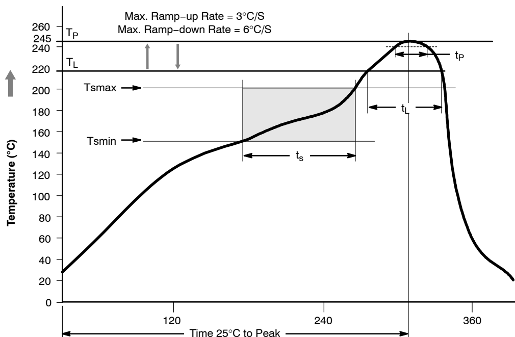
Figure 11. Reflow Profile
