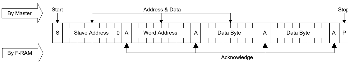
Figure 9. Multi-Byte Write
