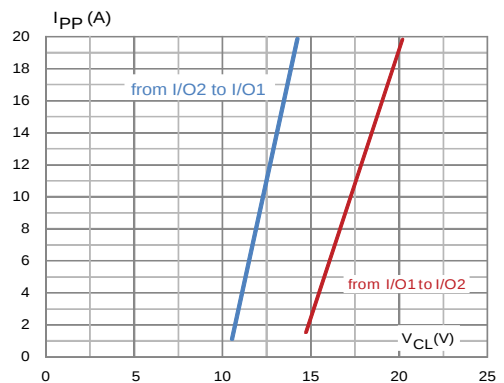
Figure 14: TLP measurement
