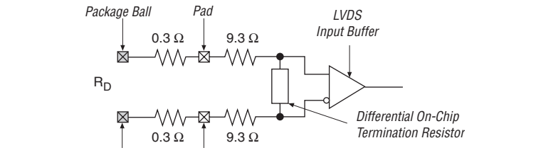
Figure 2–72. Differential Resistance of LVDS Differential Pin Pair ( R_D )
