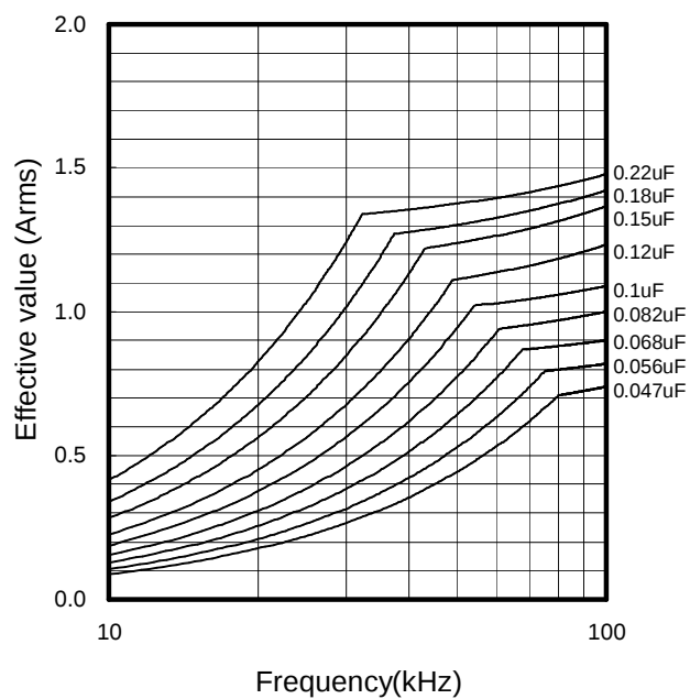
Permissible Current
