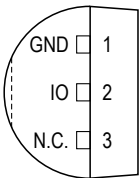
TO-92
