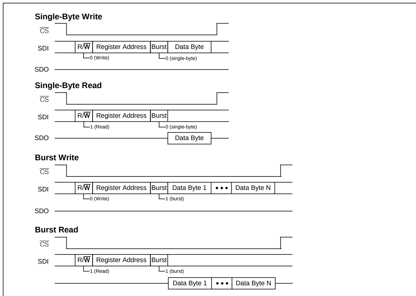
Figure 7-6. SPI Bus Transactions
