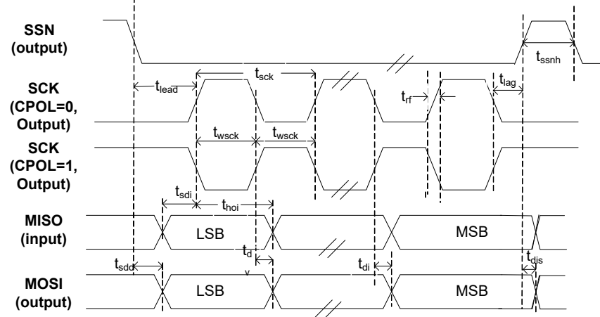
Figure 10. SPI Timing
