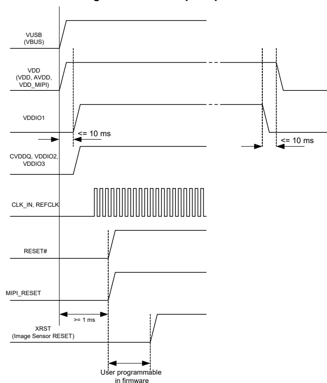
Figure 4. Power-up Sequence
