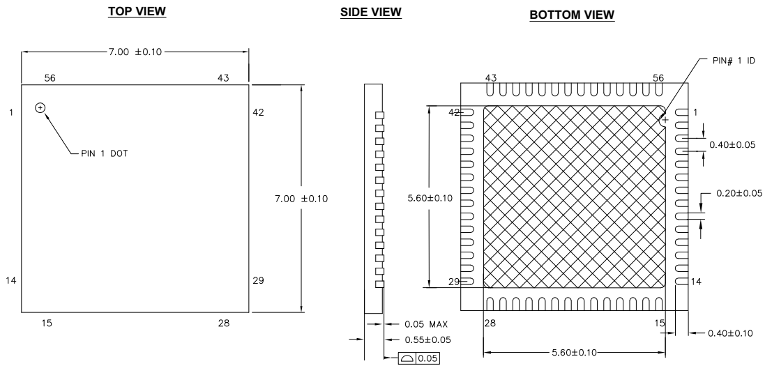
Figure 8. 56-Pin QFN 7 mm × 7 mm × 0.6 mm
