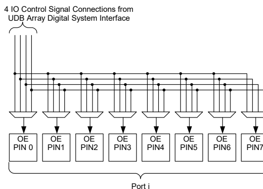
Figure 7-13. I/O Pin Output Enable Connectivity
