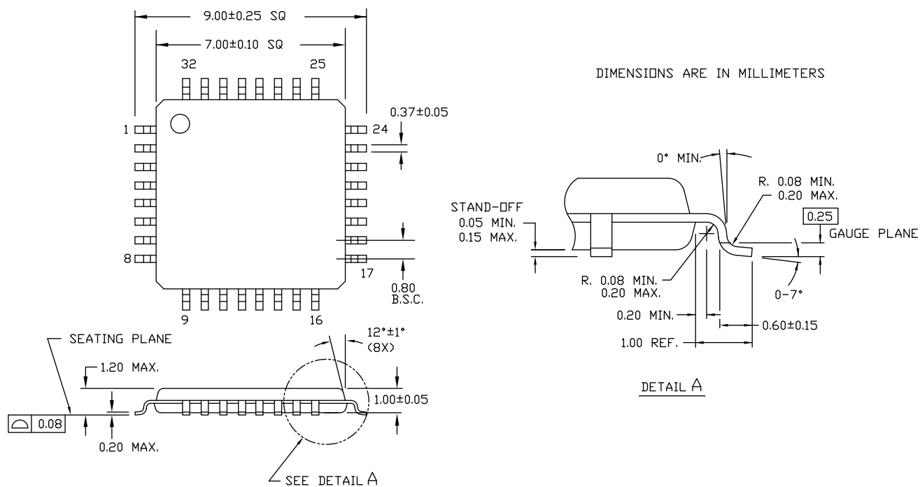
Figure 15. 32-pin TQFP (7 × 7 × 1.0 mm) A3210 Package Outline, 51-85063
