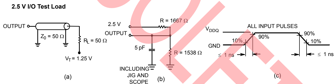
Figure 4. AC Test Loads and Waveforms
