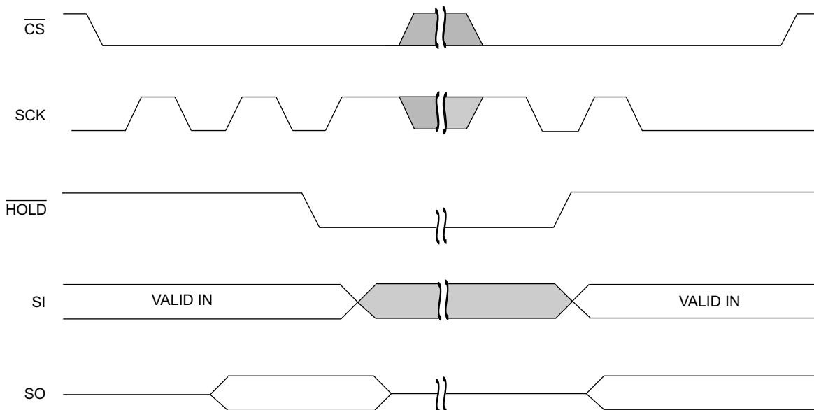
Figure 12. \overline{\text{HOLD}} Operation [2]
