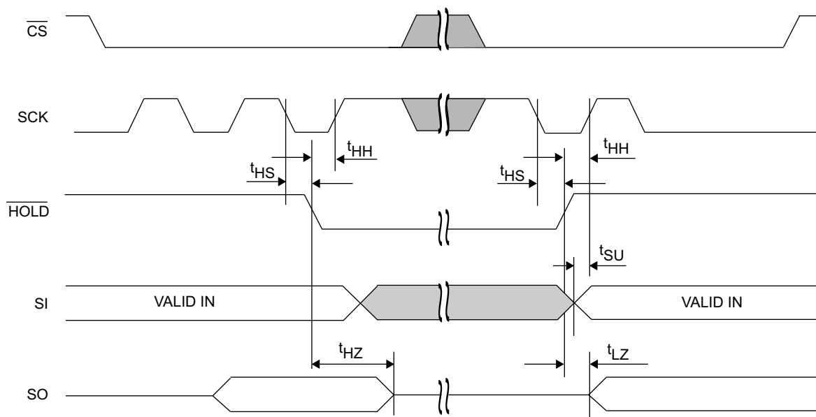
Figure 14. \overline{HOLD} Timing
