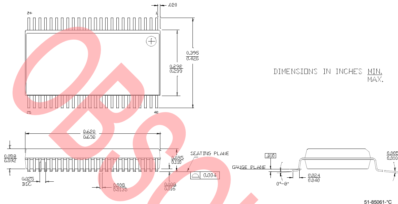
Figure 15. 48-Pin (300 mil) Shrunk Small Outline Package (51-85061)
