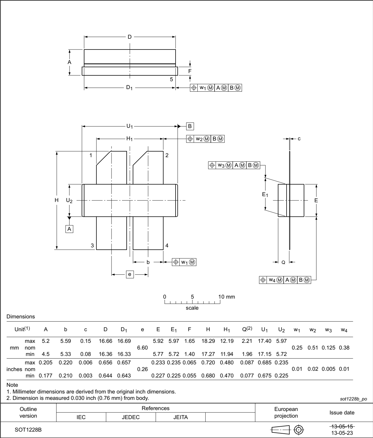
Fig 11. Package outline SOT1228B
