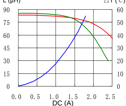
19. CDRH124NP-151MC
