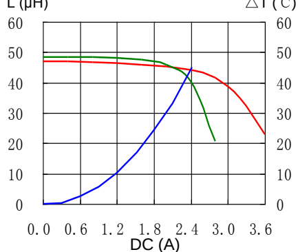
16. CDRH124NP-820MC
