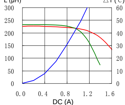
21. CDRH124NP-221MC
