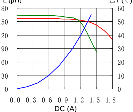
22. CDRH124NP-271MC
