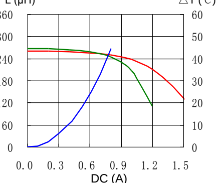
22. CDRH124NP-271MC
