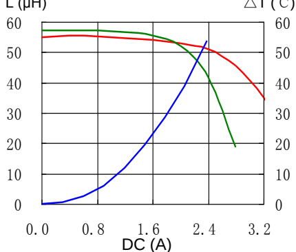
17. CDRH124NP-101MC
