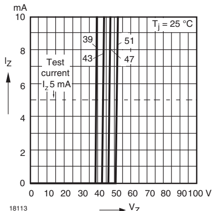
Fig. 16 - Breakdown Characteristics
