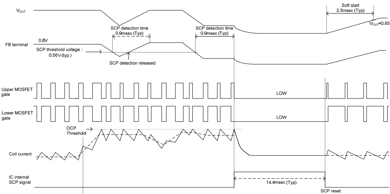
Figure 36. Short circuit protection function (SCP) timing chart
