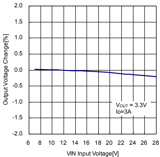
Figure 28. VOUT Line Regulation (VOUT = 3.3V)
