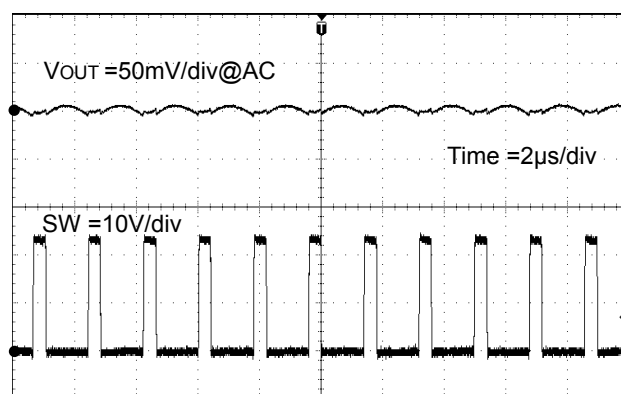
Figure 42. V_{OUT} Ripple ( V_{IN}=24V , V_{OUT}=5V , R_3=10k\Omega )
