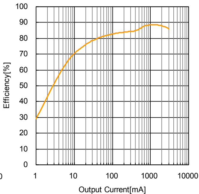
Figure 40. Efficiency - Output Current ( V_{IN}=24V , V_{OUT}=5.0V , R_3=10k\Omega )
