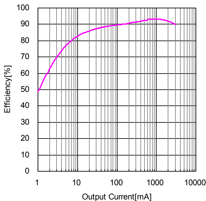
Figure 48. Efficiency - Output Current ( V_{IN}=12V , V_{OUT} = 5.0V , R3=15k\Omega , C1=18pF )
