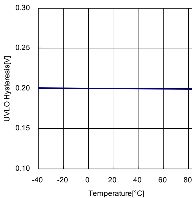
Figure 13. UVLO Hysteresis- Temperature
