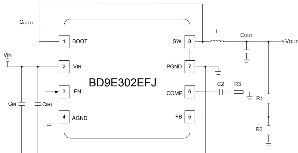
Figure 56. Application Circuit 3
