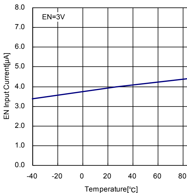
Figure 15. EN Input Current - Temperature
