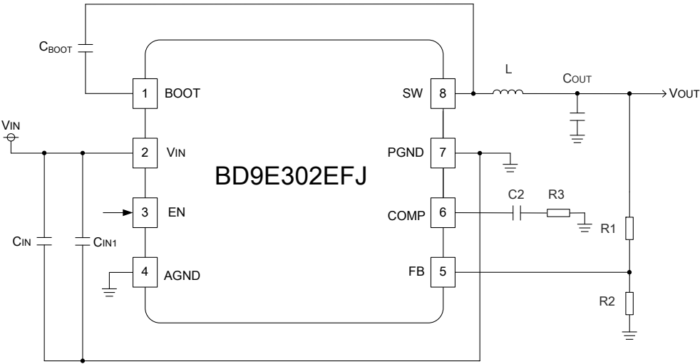
Figure 38. Application Circuit 1
