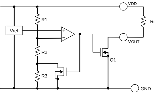
Fig.12 (BD48xxx series Internal Block Diagram)
