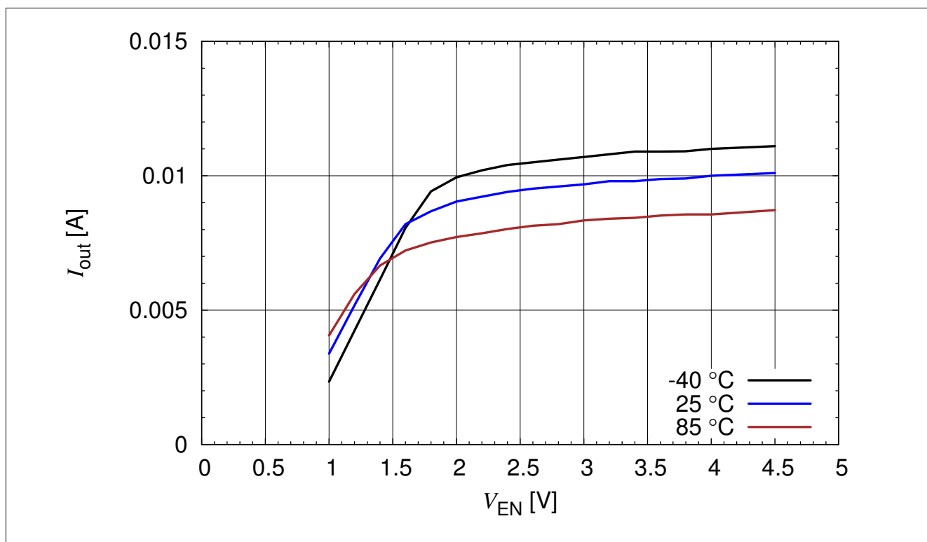
Figure 3-19 BCR 421U: Output Current versus V_{EN} I_{out} = f(V_{EN}) , V_{out} = 2 \text{ V} , R_{ext} = \text{open} , T_A = \text{Parameter}
