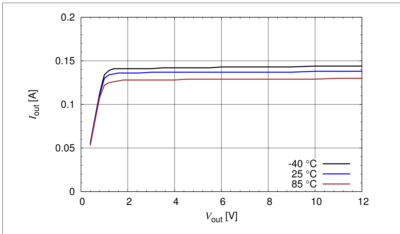
Figure 3-18 BCR 421U: Output Current versus V_{out} I_{out} = f(V_{out}) , V_{EN} = 3.3 \text{ V} , R_{ext} = 6 \Omega , T_A = \text{Parameter}
