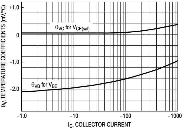
Figure 7. Temperature Coefficients
