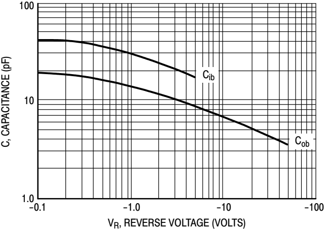
Figure 8. Capacitances
