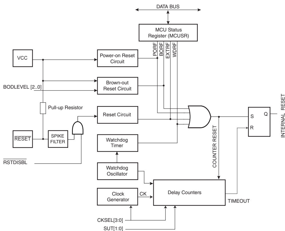
Figure 8-1. Reset Logic
