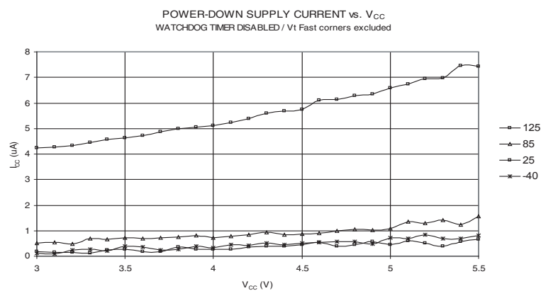
Figure 28-3. Power-Down Supply Current vs. V_{CC} (Watchdog Timer Disabled)
