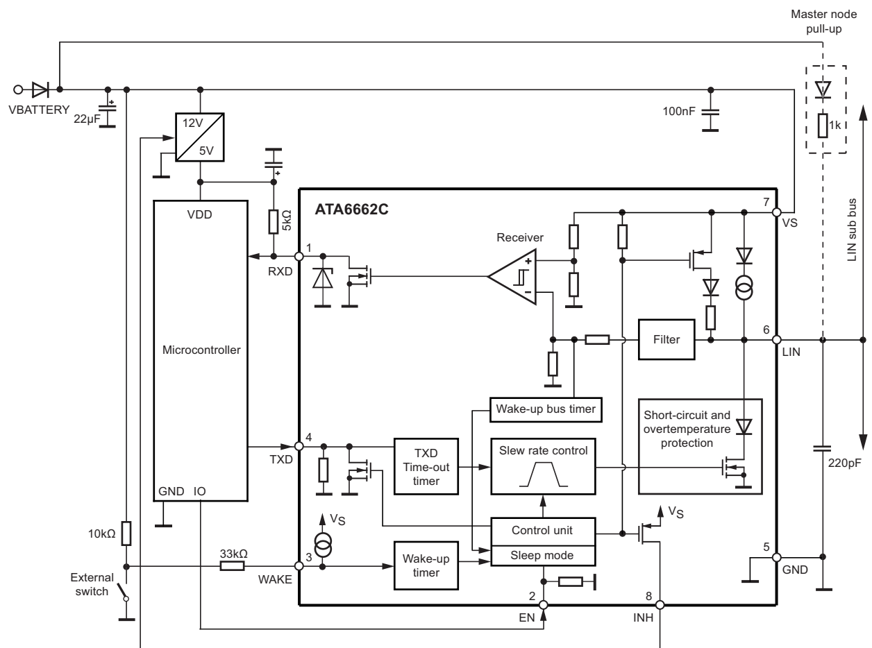
Figure 6-2. Application Circuit
