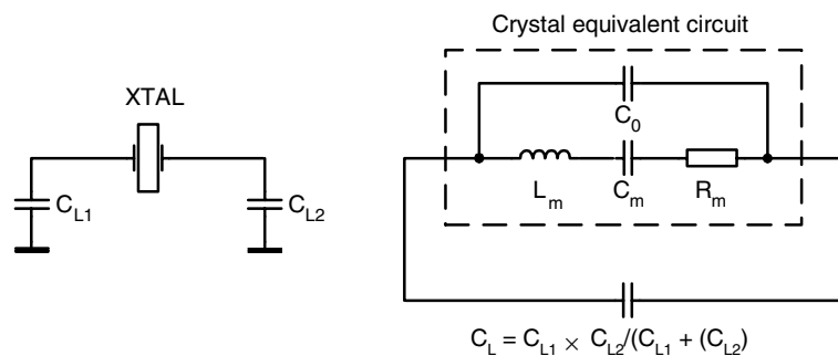
Figure 18. XTAL with Load Capacitance
