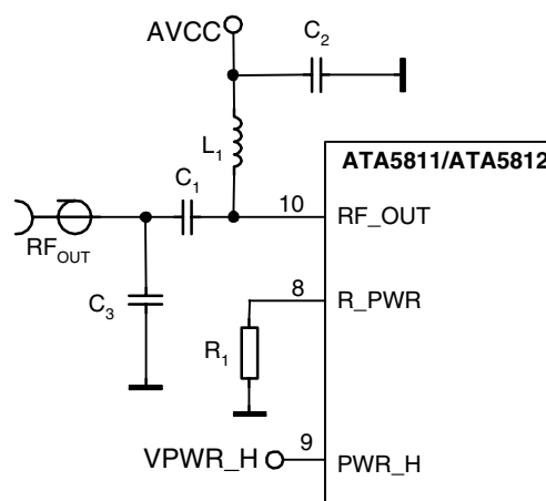
Figure 16. Power Setting and Output Matching
