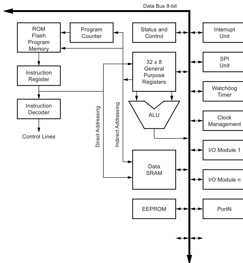
Figure 3-3. Architectural Overview
