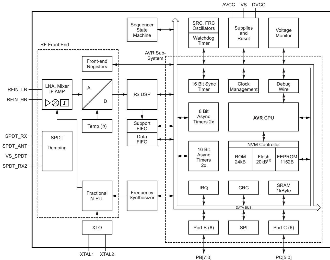
Figure 3-1. Block Diagram
