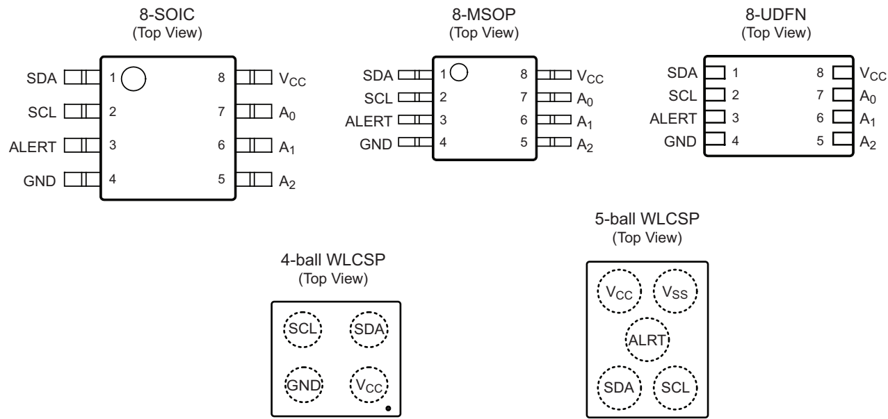
Figure 1. Pin Configurations
