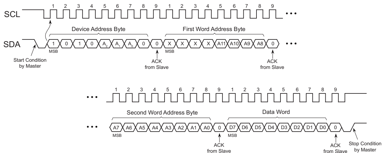
Figure 5-1. Byte Write
