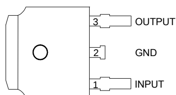
TO-252-2 (3) (Option 2)
