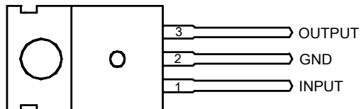
TO-220-3 (2)
