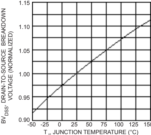
FIGURE 6, BREAKDOWN VOLTAGE vs TEMPERATURE
