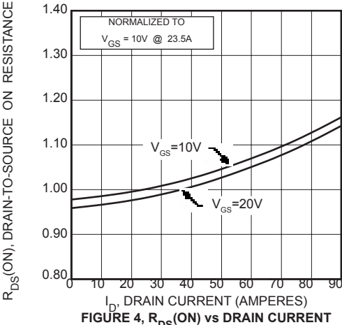
FIGURE 4, R_{DS}(\text{ON}) vs DRAIN CURRENT
