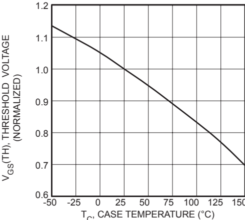
FIGURE 8, THRESHOLD VOLTAGE vs TEMPERATURE
