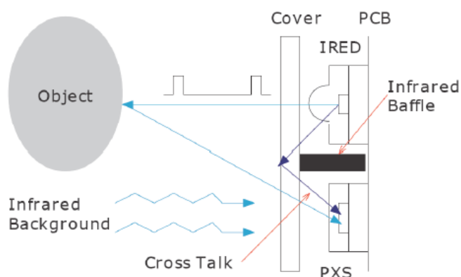
Figure 5. Proximity Sensing
