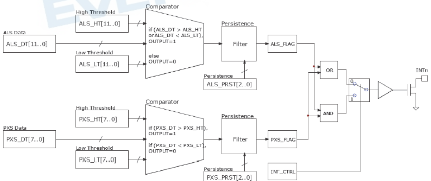
Figure 6. Interrupt operation
