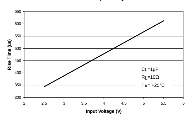
Rise Time vs Input Voltage
