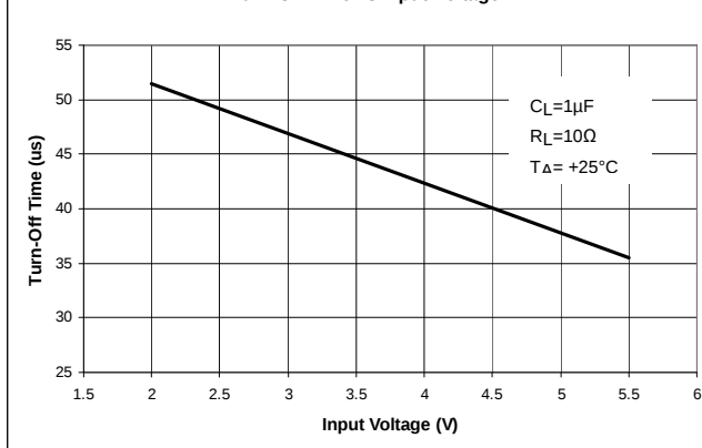
Turn-Off Time vs Input Voltage
