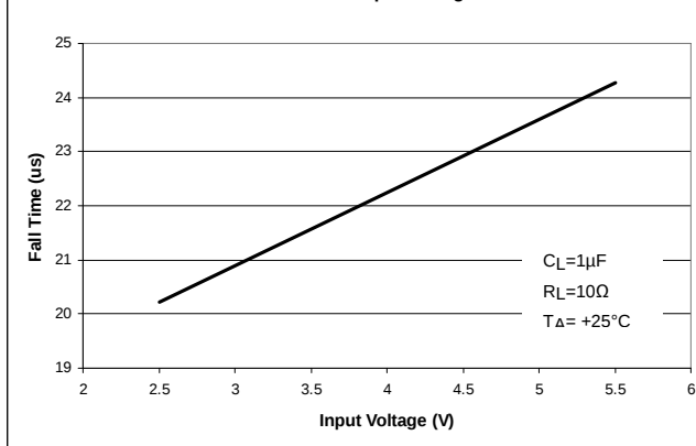
Fall Time vs Input Voltage
