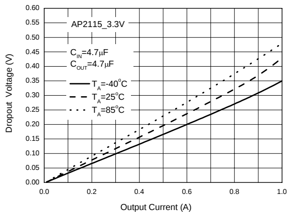
Figure 20. Dropout Voltage vs. Output Current
