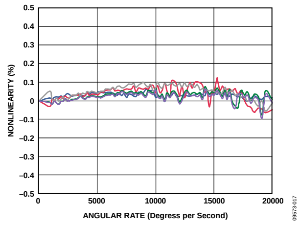
Figure 17. Typical Nonlinearity (Four Typical Devices)
