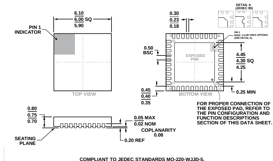
Figure 29. 40-Lead Lead Frame Chip Scale Package [LFCSP] 6 mm × 6 mm Body and 0.75 mm Package Height (CP-40-10) Dimensions shown in millimeters
