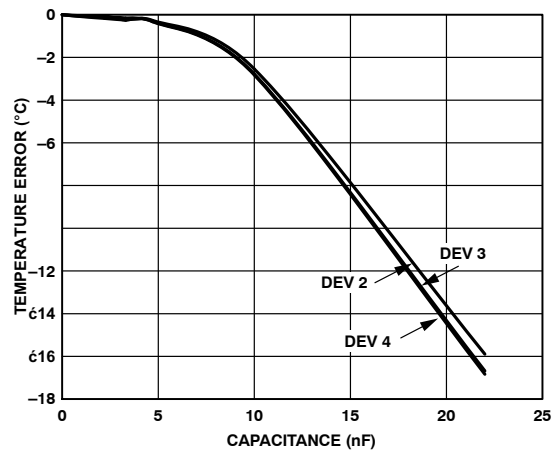
Figure 7. Temperature Error vs. D+/D- Capacitance
