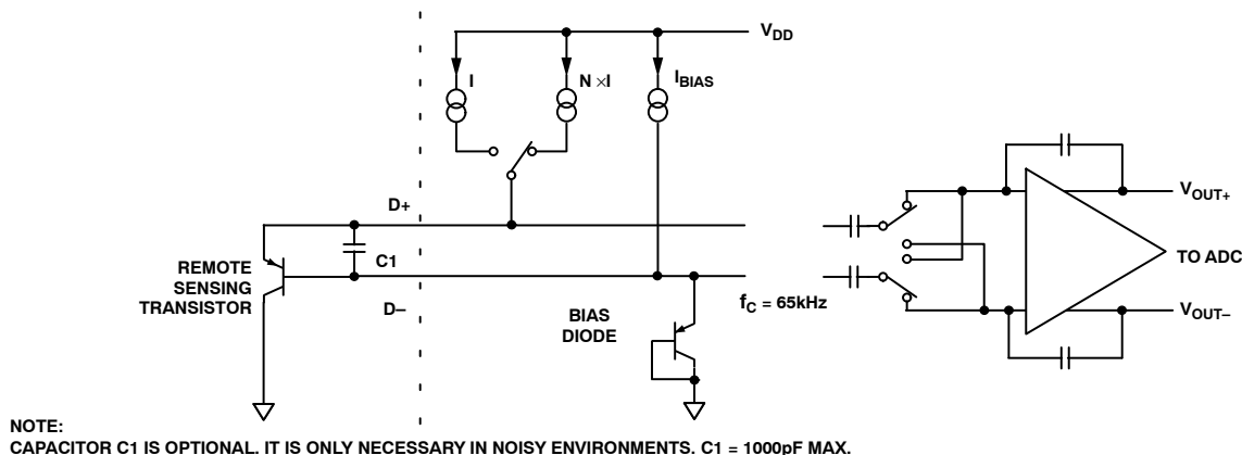
Figure 14. Input Signal Conditioning
