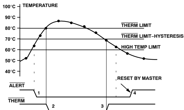
Figure 19. Operation of the \overline{\text{ALERT}} and \overline{\text{THERM}} Interrupts
