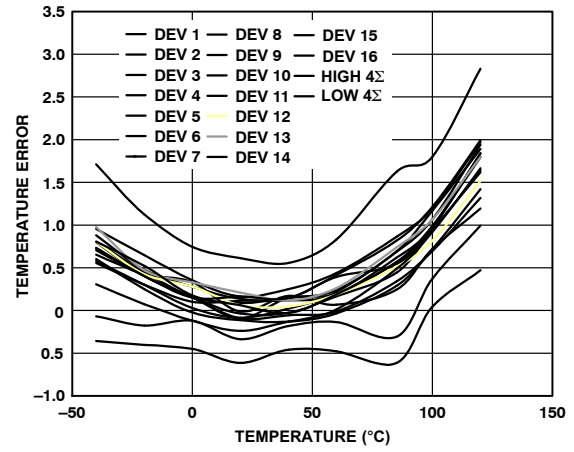
Figure 4. Remote 1 Temperature Error vs. Temperature
