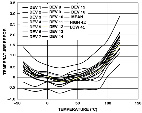
Figure 5. Remote 2 Temperature Error vs. Temperature
