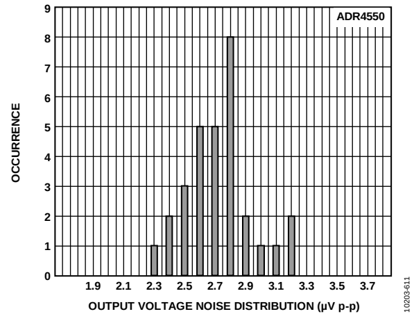
Figure 95. ADR4550 Output Voltage Noise (Maximum Amplitude from 0.1 Hz to 10 Hz)
