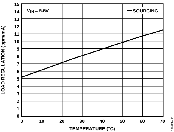
Figure 84. ADR4540 D Grade Load Regulation vs. Temperature (Sourcing)
