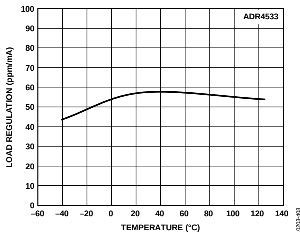
Figure 56. ADR4533 Load Regulation vs. Temperature (Sinking)
