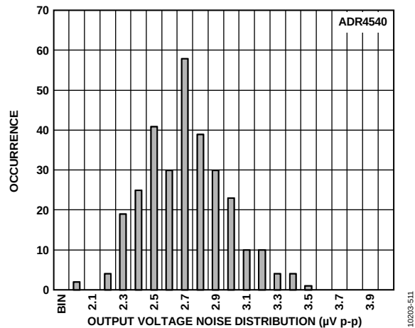
Figure 74. ADR4540 Output Voltage Noise (Maximum Amplitude from 0.1 Hz to 10 Hz)
