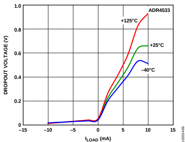
Figure 54. ADR4533 Dropout Voltage vs. Load Current
