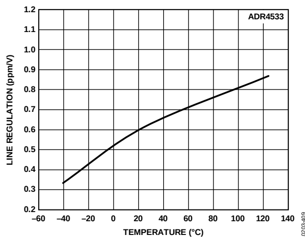
Figure 57. ADR4533 Line Regulation vs. Temperature
