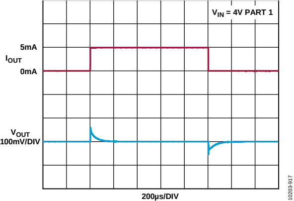
Figure 36. ADR4525 D Grade Load Transient Response (Sinking)
