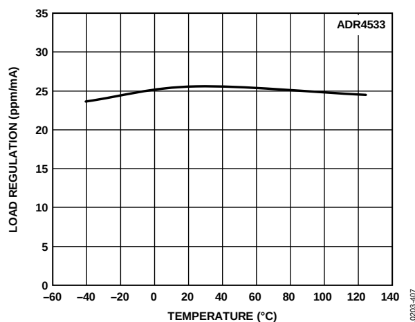
Figure 55. ADR4533 Load Regulation vs. Temperature (Sourcing)
