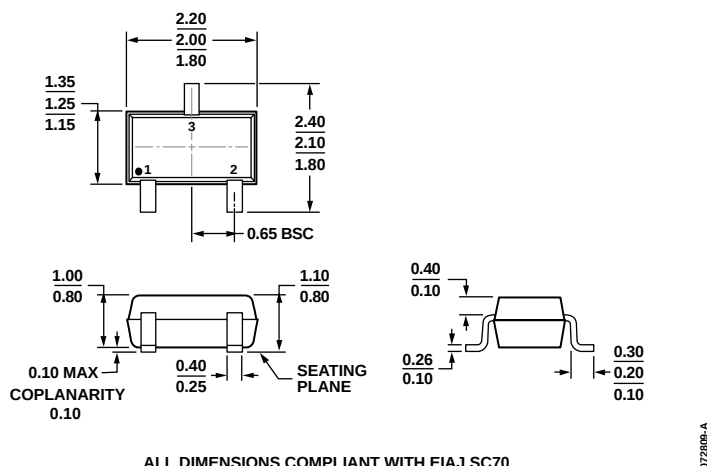
Figure 24. 3-Lead Thin Shrink Small Outline Transistor Package [KS-SC-70] (KS-3) Dimensions shown in millimeters
