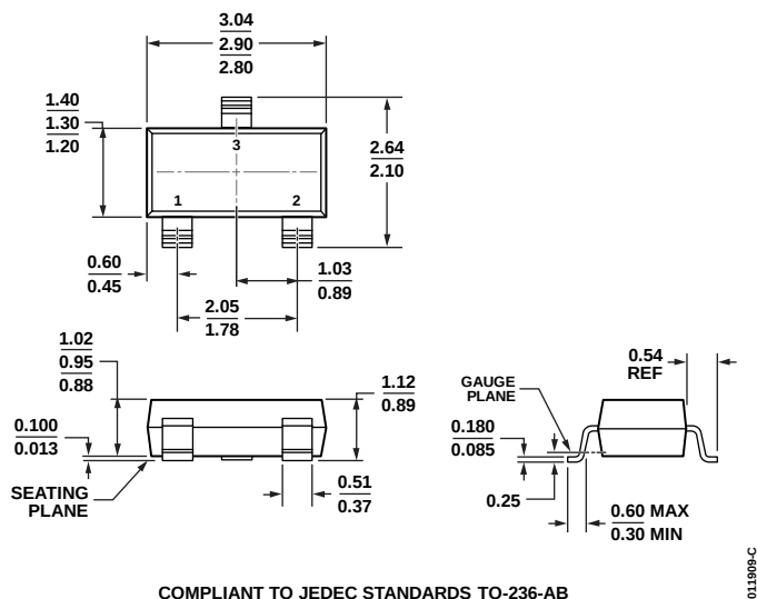
Figure 25. 3-Lead Small Outline Transistor Package [RT-SOT-23-3] (RT-3) Dimensions shown in millimeters
