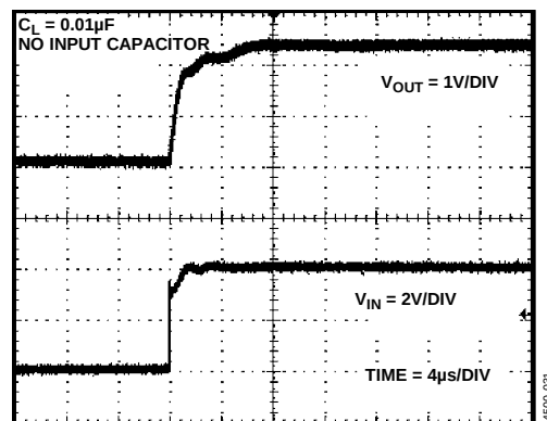
Figure 20. ADR431 Turn-On Response Settling Time, 0.01 µF Load Capacitor
