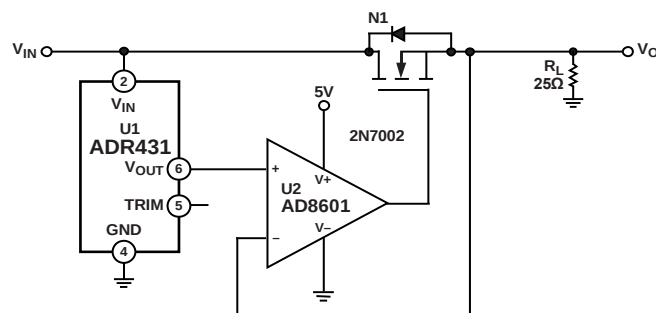
Figure 45. Precision Boosted Output Regulator
