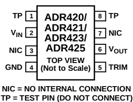
Figure 2. 8-Lead SOIC, 8-Lead MSOP Pin Configuration
