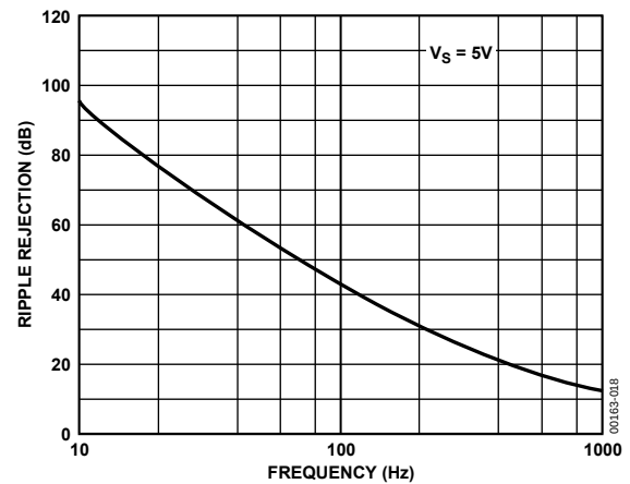
Figure 21. ADR291/ADR292 Ripple Rejection vs. Frequency
