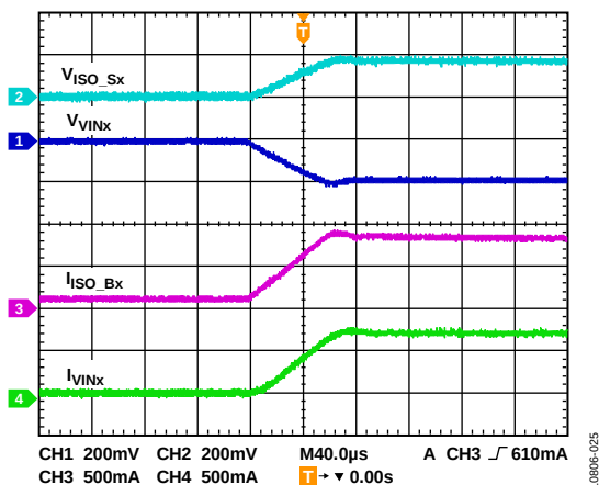
Figure 25. Input Current-Limit Transition from 100 mA to 900 mA, \text{ISO\_Sx Load} = 66\Omega , Charging = 750 mA
