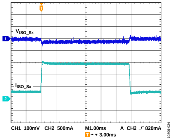
Figure 24. Load Transient, \text{ISO\_Sx Load} = 300\text{mA to }1500\text{mA to }300\text{mA}
