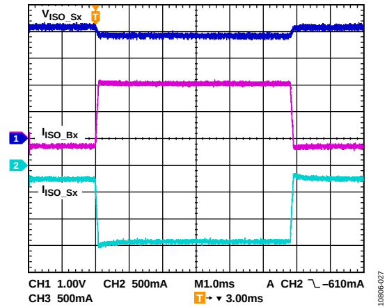
Figure 27. Load Transient, \text{ISO\_Sx Load} = 300\text{mA to }1500\text{mA to }300\text{mA} , \text{EN\_CHG} = \text{High} , \text{ILIM}[3:0] = 0110 (Binary) = 500 mA
