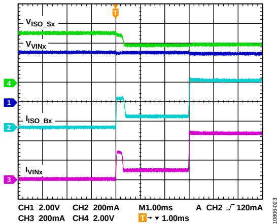
Figure 23. Charging Startup, V_{\text{VINx}} = 5.0\text{V} , \text{ILIM}[3:0] = 0110 (Binary) = 500 mA, \text{ICHG}[4:0] = 01110 (Binary) = 750 mA
