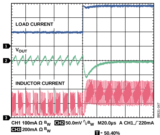
Figure 47. Load Transient, V_{OUT} = 1.2 V, 100 mA to 300 mA, Load Current Rise Time = 200 ns, V_{IN} = 5 V
