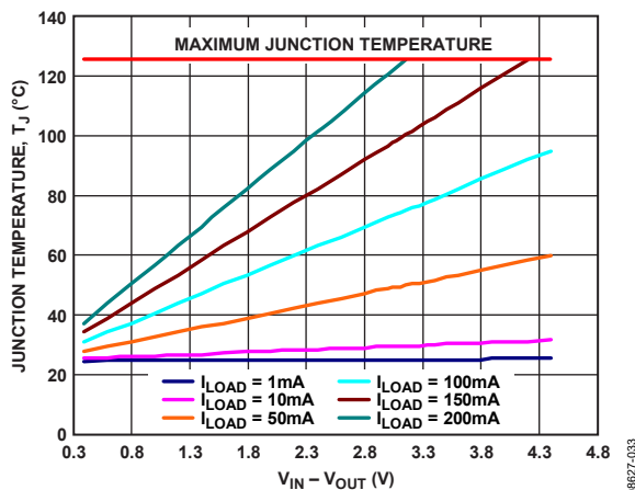
Figure 41. WLCSP 50 mm 2 of PCB Copper, T_A = 25^\circ\text{C}
