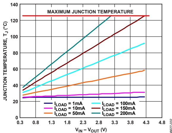
Figure 40. WLCSP 100 mm 2 of PCB Copper, T_A = 25^\circ\text{C}
