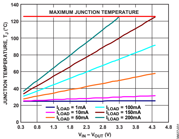
Figure 39. WLCSP 500 mm 2 of PCB Copper, T_A = 25^\circ\text{C}
