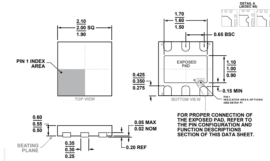
Figure 65. 6-Lead Lead Frame Chip Scale Package [LFCSP], 2.00 mm x 2.00 mm Body and 0.55 mm Package Height (CP-6-3)
