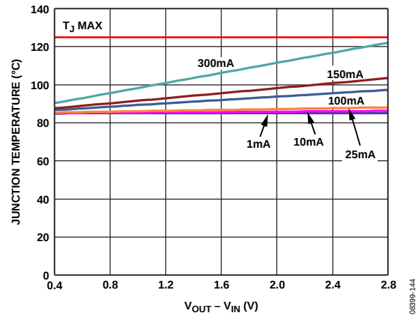
Figure 51. Junction Temperature vs. Power Dissipation, Board Temperature = 85^\circ\text{C}
