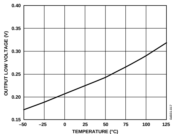
Figure 10. Receiver Output Low Voltage vs. Temperature
