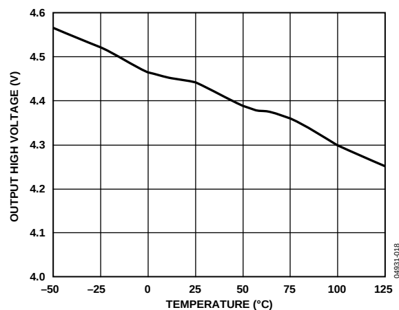
Figure 11. Receiver Output High Voltage vs. Temperature
