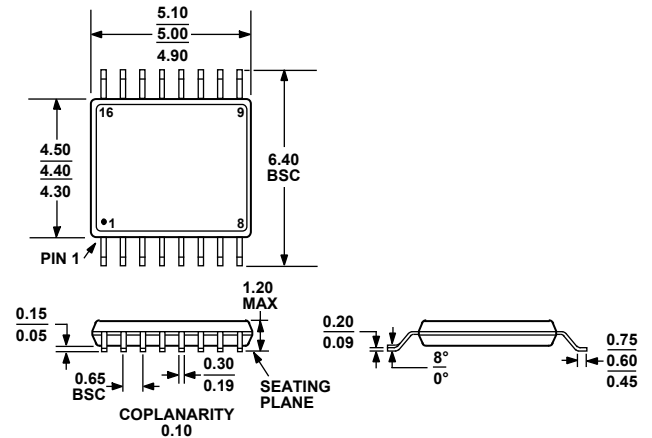
Figure 25. 16-Lead Thin Shrink Small Outline Package [TSSOP] (RU-16)
