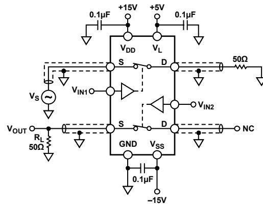
Figure 23. Channel-to-Channel Crosstalk
