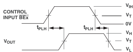
Figure 2. Propagation Delay
