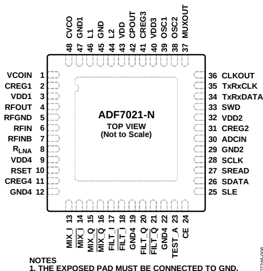
Figure 10. Pin Configuration
